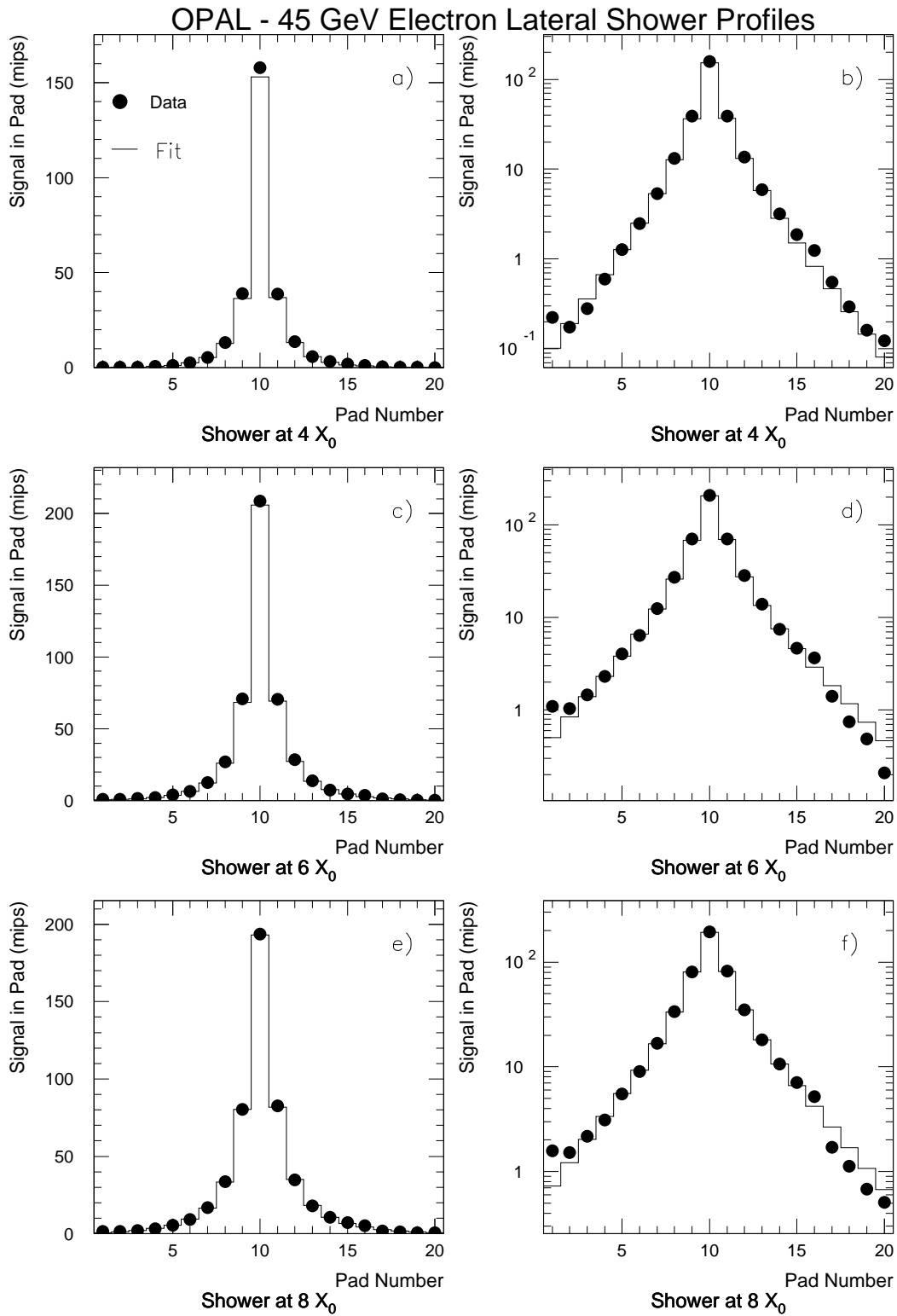
Figure 6: Average radial shower profiles at 4 X_0 a) and b), 6 X_0 c) and d), and 8 X_0 (e) and (f). The fit shows the parameterization of the electromagnetic showers given in reference [17]. The left plots show the data on a linear scale, the right plots on a logarithmic scale.
