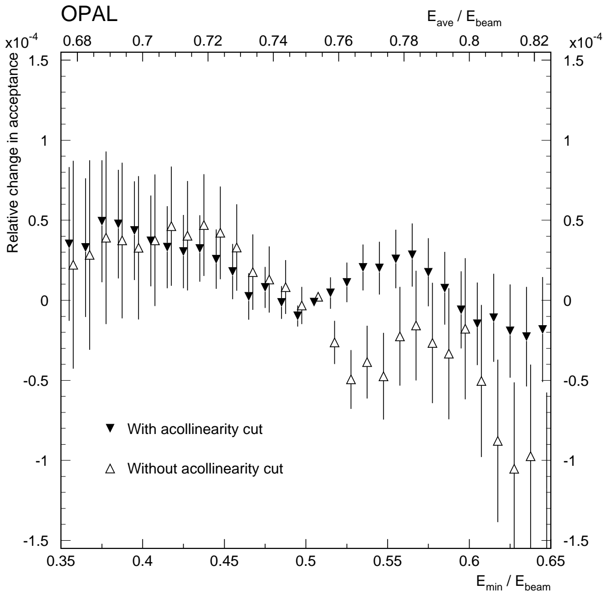
Figure 23: The relative change in acceptance between the Monte Carlo and the 1993–1994 data as a function of scaling the energy cut. The observed deviations are well within the systematic error assigned to detector energy response. The error bars show the binomial uncertainties with respect to the standard cut values.
