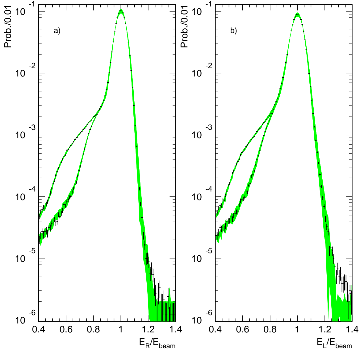
Figure 31: The normalized energy distributions in the right (a) and left (b) calorimeter for events passing all geometric cuts for the SWITA selection and which in addition have more than 0.85 of the beam energy in the opposite calorimeter. The energy spectrum is shown respectively before and after the acollinearity cut has been applied in the upper and lower branches of the curves. The points with errors show the data. The shaded bands show the Monte-Carlo predictions for the range of energy parameterizations used in assessing the systematic error (see section 4.3). Above 0.8 the upper and lower branches of the curves are nearly indistinguishable.
