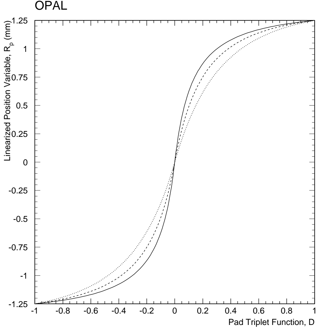
Figure 9: The linearized position variable, R_p , in millimeters as a function of D , in units of half pad widths. This is shown for characteristic shower depths of 4 (solid line), 6 (dashed line) and 8 X_0 (dotted line). The center of the pad is at 0, and the boundaries at \pm 1.25 mm.
