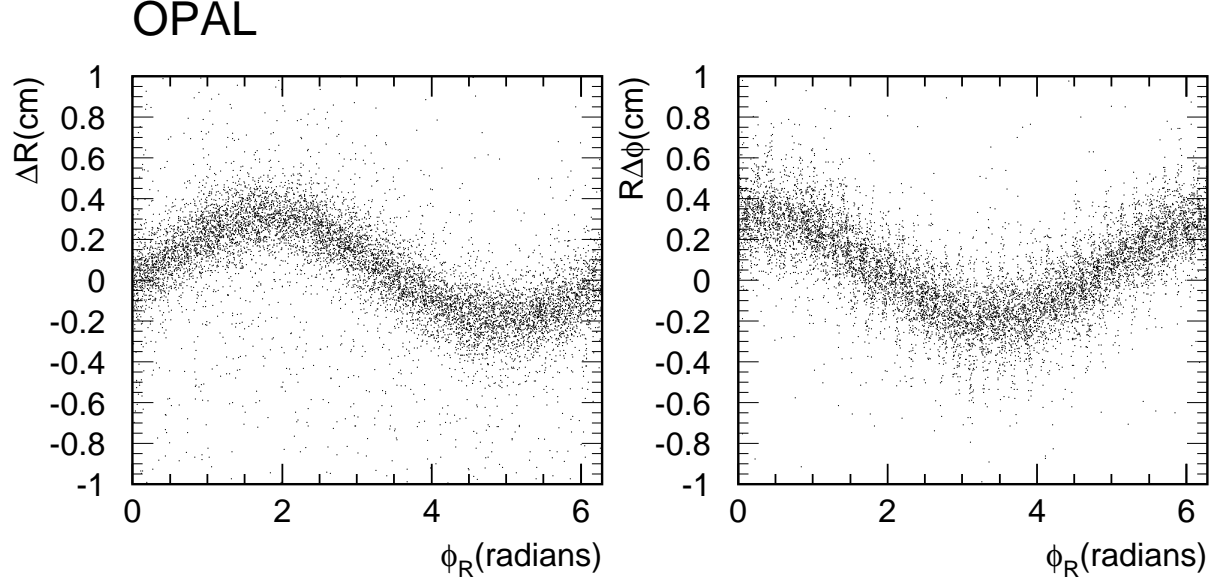
Figure 28: The beam spot position can be determined with great precision from the measured coordinates of back-to-back Bhabha clusters. The plot on the left shows the acollinearity of non-radiative Bhabhas in the detector frame as a function of \phi_R . The plot on the right shows R times acoplanarity for the same sample.
