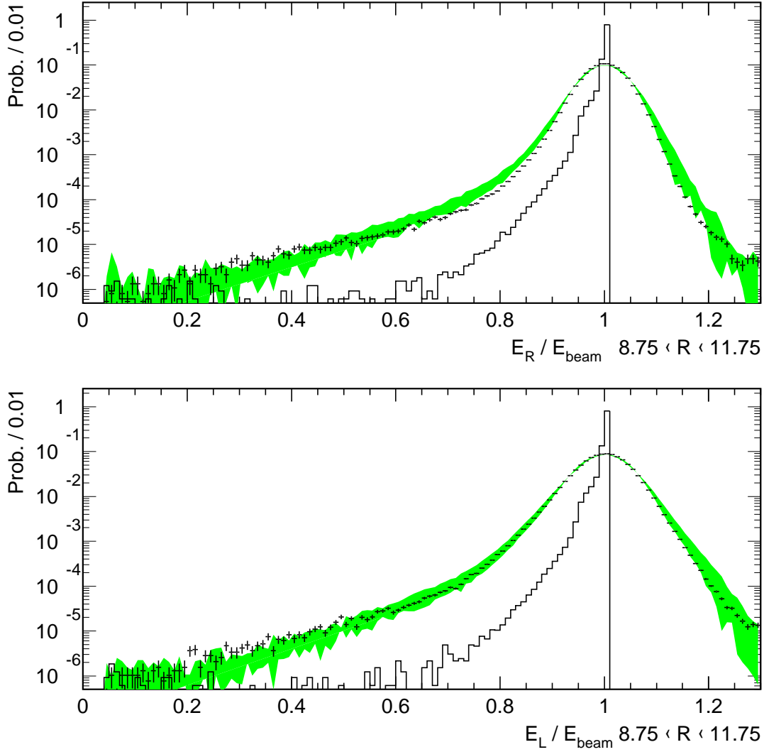
Figure 21: The observed detector energy response to very collinear events, with |R_R - R_L| < 1 mm, (points) which is used to parameterize the detector simulation (shaded band) for showers in the radial region between 8.75 and 11.75 cm. The width of the shaded band shows the variation in the parametrization used in setting the systematic error. Because of the tight acollinearity cut applied to the samples, single radiative and double radiative events are highly suppressed, and the observed distribution is dominated by resolution effects, as illustrated by the narrow histogram of the bare BHLUMI four-vectors, whose tail falls two orders of magnitude below the simulated detector response.
