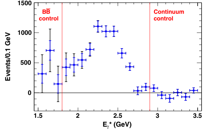
FIG. 1 (color online). The measured E_\gamma^* photon energy spectrum after background subtraction, uncorrected for efficiency and resolution smearing. The inner error bars are statistical only, while the outer include systematic errors added in quadrature.
