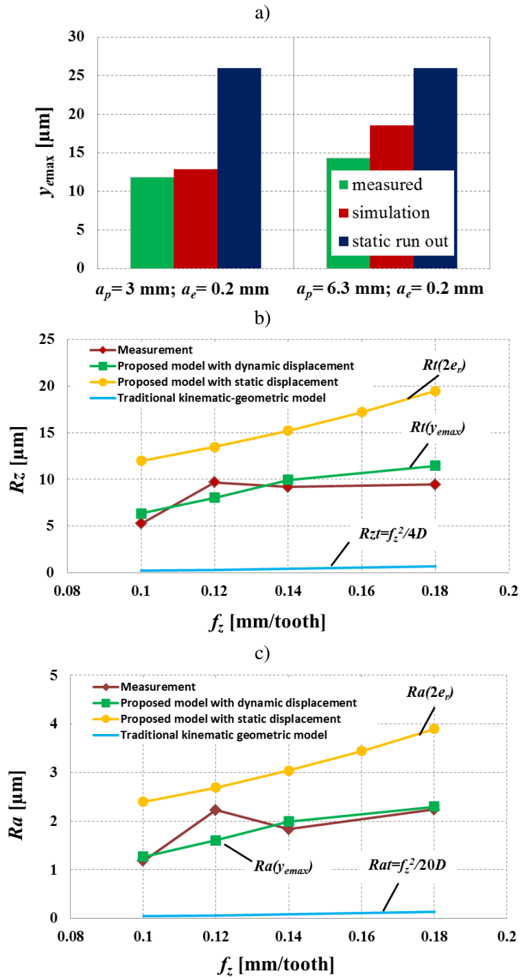
Fig. 11. The comparison of measured and calculated values ( a_p = 3 \text{ mm} ) of: a) height of cutter's displacement envelope y_{max} , b) surface roughness R_z , c) surface roughness R_a
