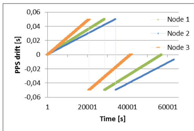
Figure 3 Clock offset between GM node and slave nodes without synchronization
