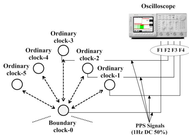
Figure 2 Illustration of the offset measurements setup
