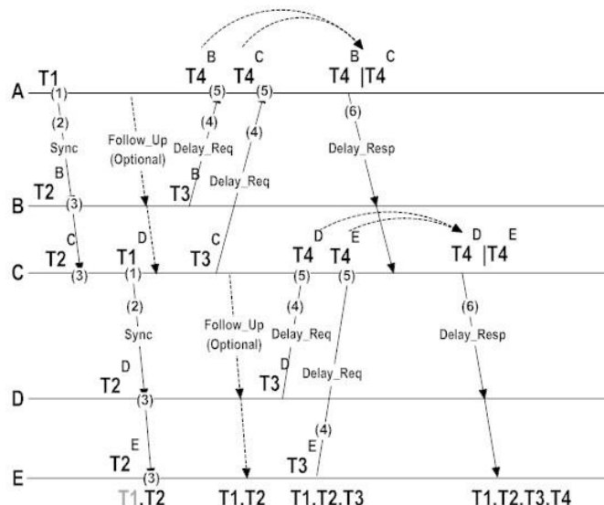
Figure 1 Synchronization message exchange for hierarchical topology. The slave node exchange PTP messages with master or boundary clock
