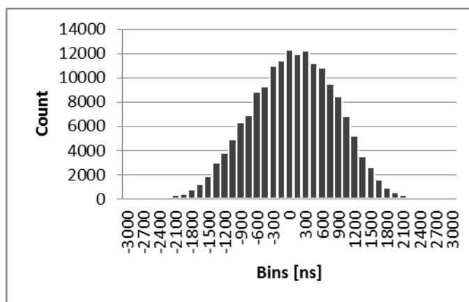
Figure 4 PPS signals delay histogram in star network with communication rate of 5s
