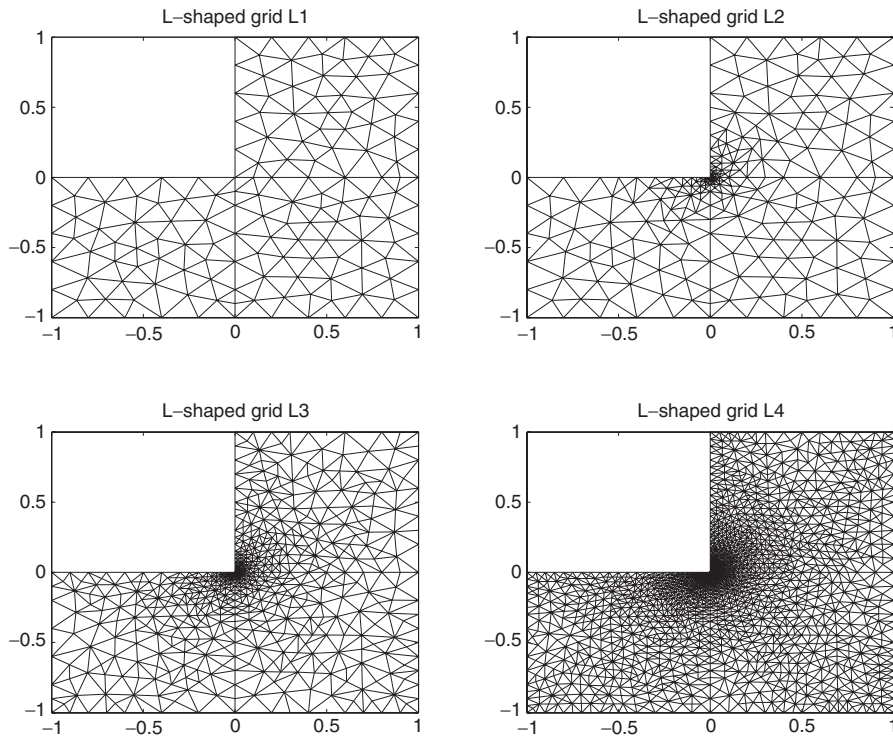
Figure 2. Grids L1–L4 for Example 6.2.
