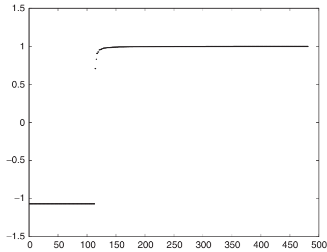
Figure 1. Plot of the eigenvalues of the preconditioned matrix \mathcal{P}_{M,L}^{-1}\mathcal{K} , for k = \frac{1}{4} , for grid G2 in Example 6.1.
