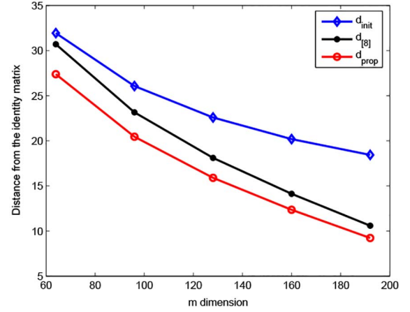
Fig. 1. Discrepancy between the Gram or pseudo-Gram matrices involved in support estimation and the identity matrix of same dimensions. The experiments involve m \times N matrices with m \in [64 : 32 : 192] and N = 256 .
