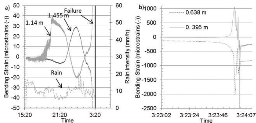
Fig. 12 a Changes in bending strain at depths of 1.14 and 1.455 m (above and below the eventual failure surfaces, respectively) along SDS 4. b Changes in the bending strain at depths of 0.395 and 0.638 m of SDS1 installed in cluster 2 during the last seconds before the failure
