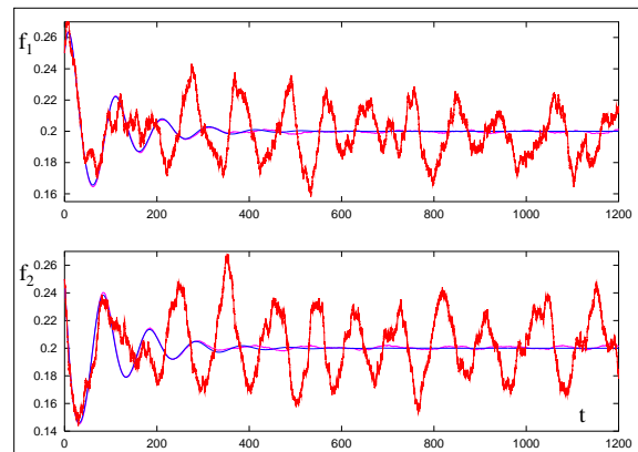
FIG. 1: Predator and prey densities as a function of time. The upper panel shows the predator density f_1 for N = 3200 . The blue line is calculated from numerical integration of the mean field Volterra Eqs. (3). The purple line is the average of the predator density time series from 500 replicates generated from the ILM, and is almost indistinguishable from the mean field solution. The red line is the predator density time series for a single typical replicate. The lower panel is the equivalent plot for the prey density f_2 . Parameter values are b = 0.5 , d_1 = 0.1 , d_2 = 0.0 , p_1 = 0.5 , and p_2 = 0.1 .
