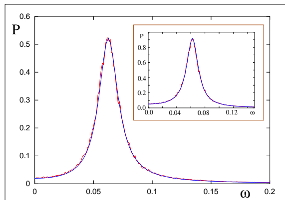
FIG. 2: A plot of the power spectrum P(\omega) for the predator time series, as a function of frequency \omega . The red line corresponds to P calculated from 500 replicate runs of the ILM. The blue line is the prediction from our theory, namely Eq. (9). The parameter values are the same as those described in the caption to Fig. 1. The inset shows the analogous power spectra (data and theory) for the prey time series.
