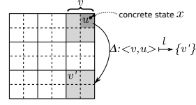
Fig. 3: Concrete state space partitioned into abstract states (solid lines) and untracked sub-states (dashed lines).
