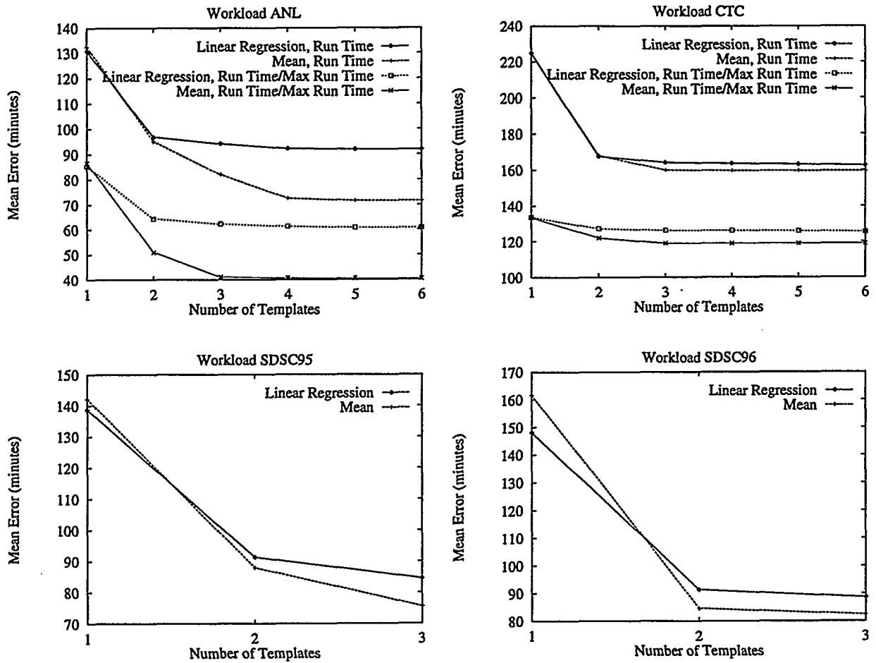
Figure 1: Mean errors of greedy searches
