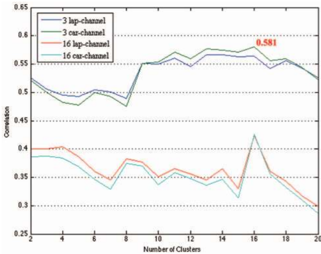
Figure 15. The changes of the correlation between the proposed predictor and the classification performance according to the number of clusters and the number of channels considered in prediction. doi:10.1371/journal.pone.0087056.g015
