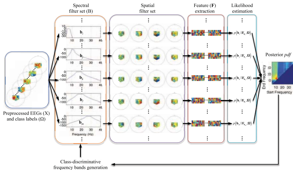
FIGURE 3. An illustration of estimating p(\mathbf{B}|\mathbf{X}, \Omega) that represents how likely the EEGs \mathbf{X} is correctly classified into the corresponding label \Omega for each of the frequency bands in \mathbf{B} .
