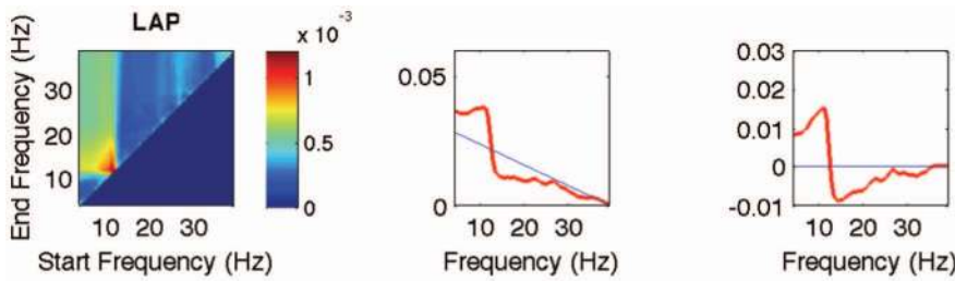
Figure 4. Estimation of a 1-dimensional pdf from a 2-dimensional pdf estimated by BSSFO. (Left) A 2-dimensional pdf estimated by BSSFO. (Middle) The red line represents the 1-dimensional pdf of the estimated 2-dimensional pdf and the blue straight line is the 1-dimensional pdf of a uniform 2-dimensional pdf. (Right) The red line is the uniform pdf subtracted version of the 1-dimensional pdf. doi:10.1371/journal.pone.0087056.g004
