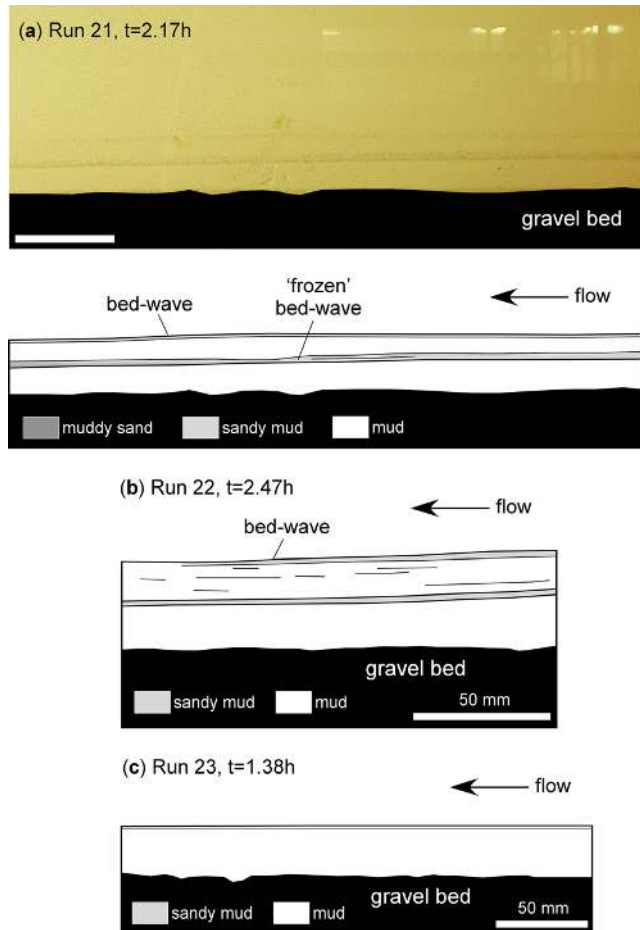
Fig. 28. WOR-equivalent bedforms in (a, b) upper transitional plug flow and (c) quasi-laminar plug flow. (a) 2.17 h, (b) 2.47 h, and (c) 1.38 h after the start of Runs 21, 22, and 23, respectively.
