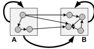
Figure 4. Lifting up dependencies
