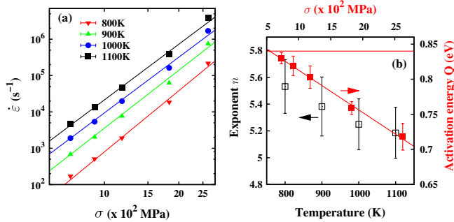
FIG. 4 (color online). (a) Creep over a range of stresses and temperatures T > 0.4T_m for reference supersaturation \rho_v^{\text{ref}}(729.9 \text{ MPa}, 1100 \text{ K}) = 10^{-4} . (b) Stress exponents and effective activation energies at different temperatures and applied stresses, respectively. The solid horizontal line represents the activation barrier of self-diffusion (0.84 eV) in a dislocation-free lattice. The effective activation energy is a linear function of applied stress, Q = Q_0 - V_a\sigma , where Q_0 = 0.87 eV. Calculated activation volume V_a = (0.85 \pm 0.03)\Omega_0 , where \Omega_0 is the Fe atomic volume, is consistent with dislocation creep controlled by vacancy diffusion.
