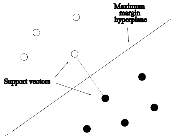
Figure 2: A small two-class dataset with nine instances and the corresponding maximum margin hyperplane
