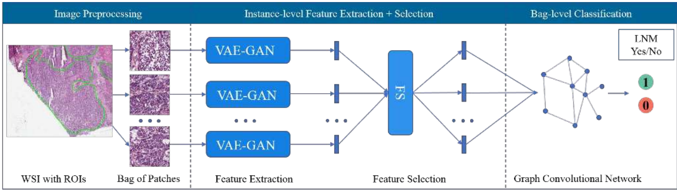
Figure 1. The overall framework of the proposed approach. It consists of image preprocessing, instance-level feature extraction, instance-level feature selection, and bag-level classification. VAE-GAN works as an instance-level feature extractor. The feature selection procedure selects discriminative instance-level features. The GCN is used to synthesize selected instance-level features, generate bag representation and perform the final classification.
