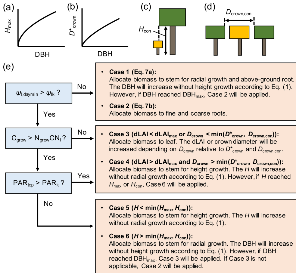
Figure 3. Schematics of (a, b) allometric and (c, d) physical constraints on tree height ( H_{max} , H_{con} ) and crown diameter ( D^*_{crown} , D_{crown,con} ), where the H_{con} and D_{crown,con} in panels (c) and (d) are for the tree with crown filled by yellow color and (e) the newly added biomass allocation scheme to SEIB-DGVM. See Note S1 for the derivation of allometric constraints from field data.
