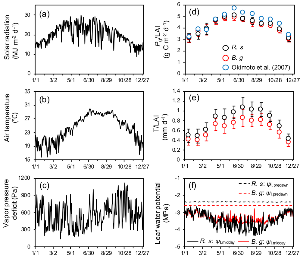
Figure 4. Seasonal variations in atmospheric forcing variables: (a) solar radiation, (b) air temperature, and (c) vapor pressure deficit (VPD). Modeled seasonal dynamics: (d) monthly mean and standard deviation of species-specific gross photosynthetic rate ( P_g , gC per square meter ground per day), (e) transpiration ( T , \text{mm d}^{-1} ) normalized by leaf layer index (LAI, \text{m}^2 \text{m}^{-2} ) of the respective species, and (f) midday ( \psi_{l,\text{midday}} ) and predawn ( \psi_{l,\text{predawn}} ) leaf water potential of each species. R. s. : R. stylosa ; B. g. : B. gymnorrhiza . Solar radiation is expressed as daily sum, while air temperature and VPD are expressed as daily mean. The leaf water potential shown is the median value of individuals. Here, the modeled dynamics are from a simulation of soil salinity set as 30‰, and the results of a year when LAI reached 1.55 are shown. At this time, the LAIs of R. stylosa and B. gymnorrhiza are 0.87 and 0.68, respectively. In panel (d), seasonal variations in P_g/\text{LAI} measured by Okimoto et al. (2007) are also shown as reference, the data of which are from an area with LAI = 1.55 in the Fukido mangrove forest in 2000–2001.
