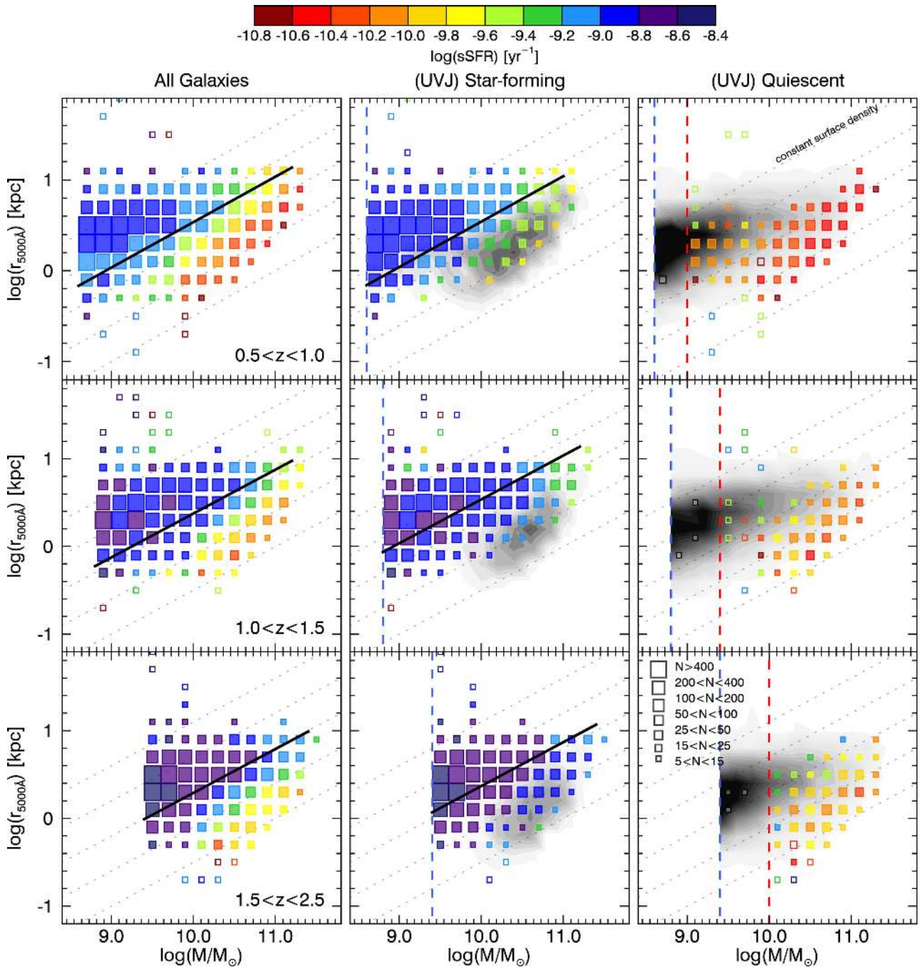
Figure 1. Rest-frame 5000 Å size of galaxies as a function of stellar mass, color-coded by the sSFRs derived from UV+IR median stacking analyses in 0.2 dex bins of \log M_*/M_\odot and \log r_{5000 \text{ \AA}} . The size of the symbol depends on the number of galaxies that enter each bin. The vertical dashed lines correspond to the stellar mass limits down to which the structural parameters can be trusted for star-forming (blue) and quiescent (red) populations. The black dotted lines correspond to lines of constant surface density, stellar mass per unit area, with the solid line corresponding to the characteristic central density measured in Figure 9.
