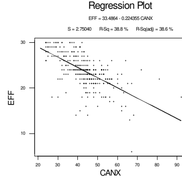
Figure 1 – Regression Plot of Software Self-Efficacy vs Computer Anxiety
