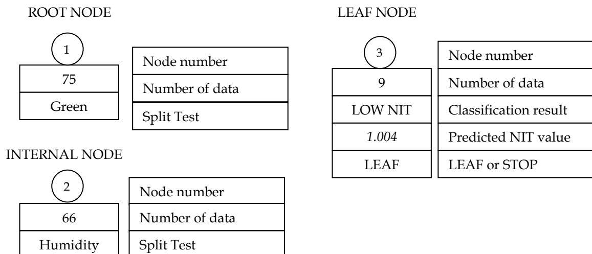
Figure 5 - Information show in decision tree nodes
