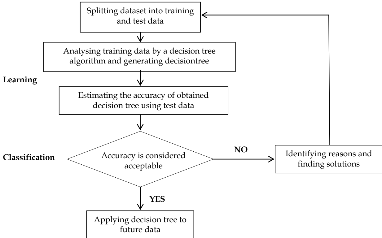
Figure 3 - Flow chart of making a decision tree (Yu et al. [18])
