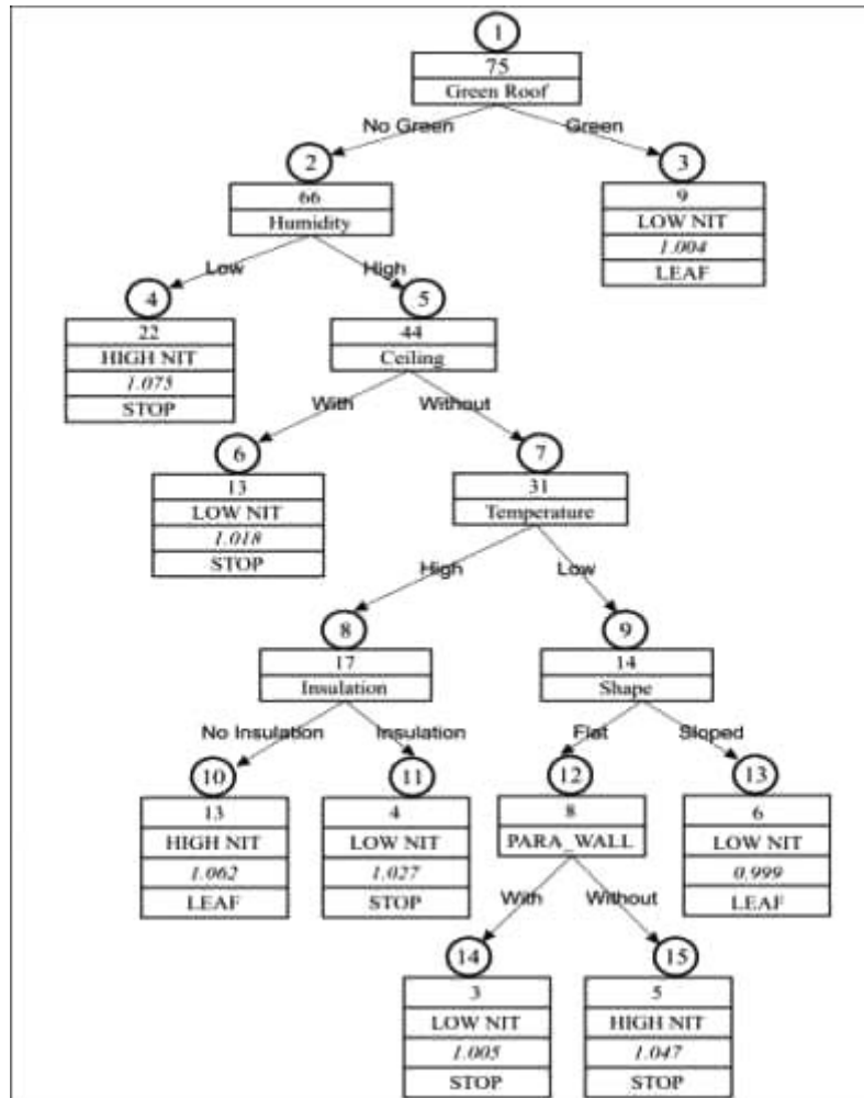
Figure 4 - Decision tree constructed by using WEKA
