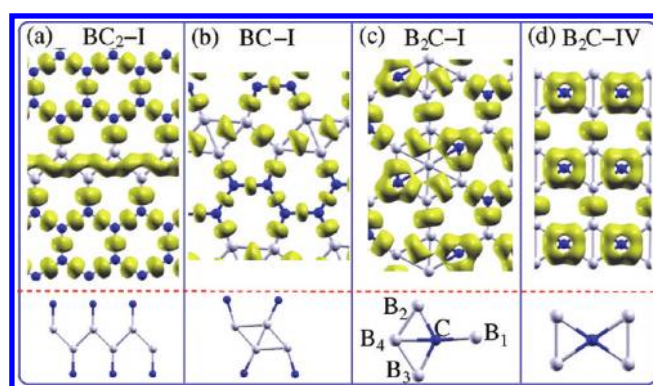
Figure 11. Isosurfaces of electron localization function with the value of 0.7 for (a) BC_2 -I, (b) BC -I, (c) B_2C -I, and (d) B_2C -IV. The structural characters are shown in the lower panels.
