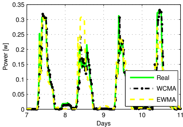
Fig. 4. Prediction accuracy of WCMA vs. EWMA
