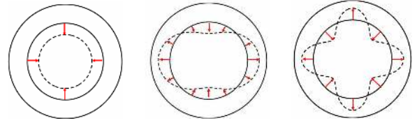
Fig. 3. Illustration of the electromagnetic force decomposition in several sinusoidal force waves (spatial orders 0, 2 and 4). The magnitude, velocity, propagation direction of these elementary force waves are given by the 2D Fourier series of the air-gap electromagnetic pressure distribution.
