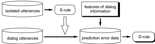
Figure 2. Flow of the S- and D-rule generation
