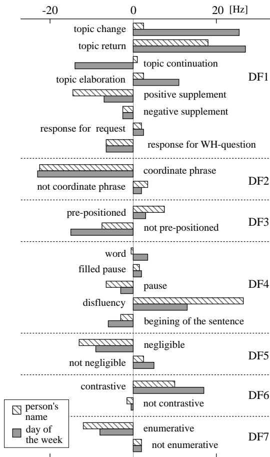
Figure 3. Model parameters of D-rule
