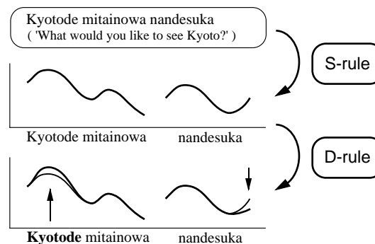
Figure 1. Two step prediction of prosody in dialogue
