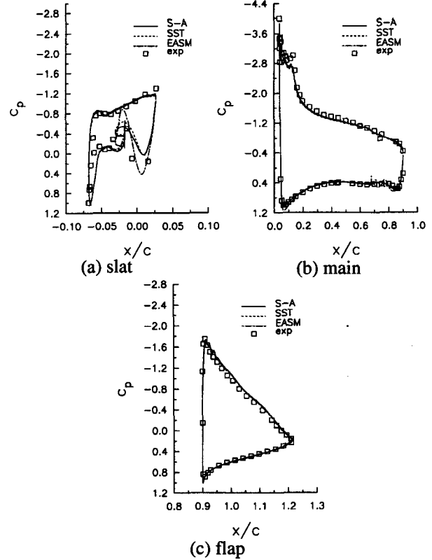
Fig. 3. AGARD surface pressure coefficient, \alpha=4.01^\circ .
