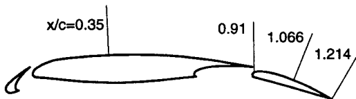
Fig. 5. AGARD profile locations.
