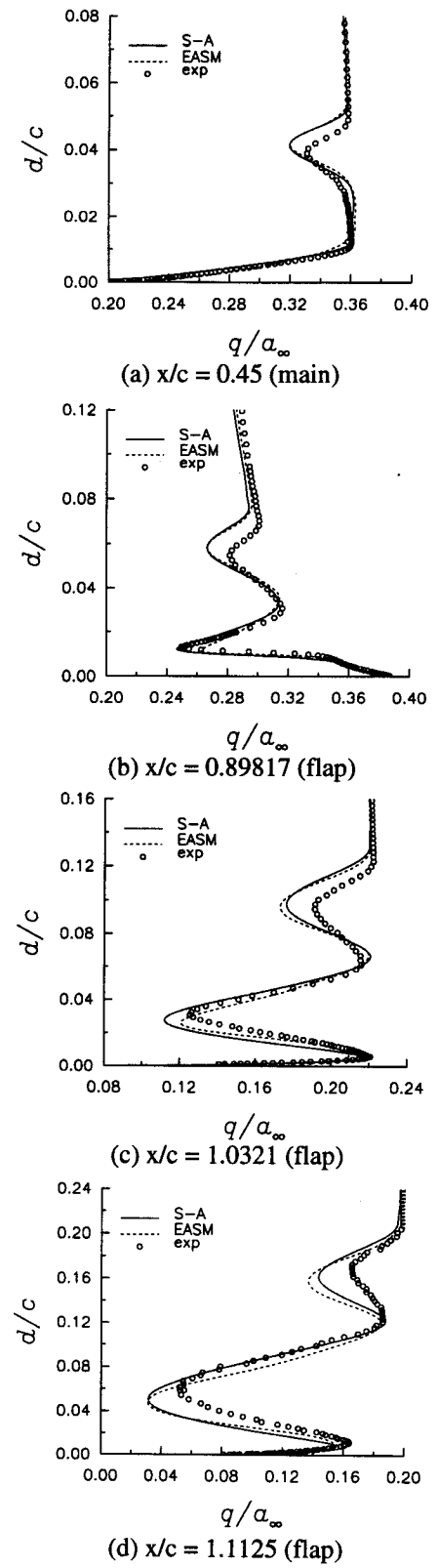
Fig. 17. Effect of turbulence model on 30P-30N velocity profiles, transition set, walls modeled, \alpha=19^\circ .
