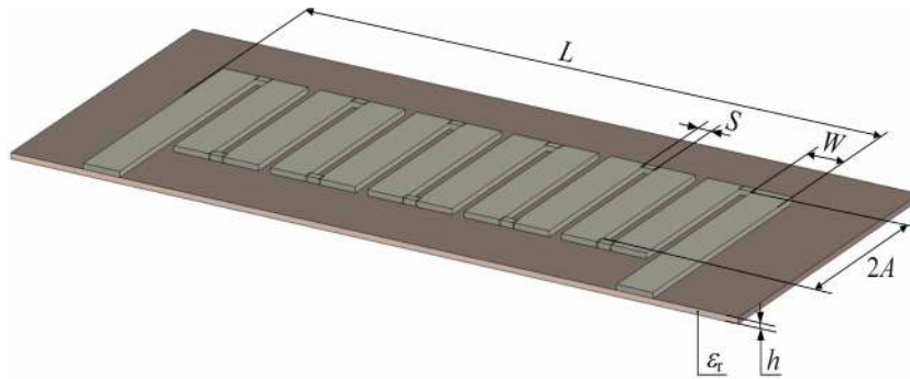
FIGURE 1. The model of the meander delay system, where h is the thickness of dielectric substrate; W is the width of the meander conductor; 2A is the length of the conductor; S is the gap between adjacent conductors; L is the length of the meander delay system; \epsilon_r is the permittivity of the dielectric substrate.
