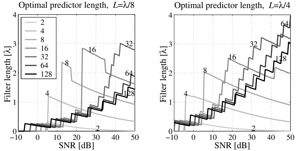
Figure 6.8: The optimal filter length (M-1)\Delta t_\lambda , for prediction of a channel tap, with Jakes spectrum, as a function of SNR, for a predictor with M = \{2, 4, \dots, 128\} coefficients.
