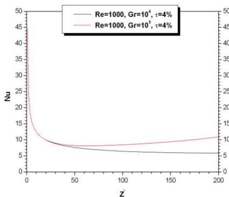
Fig. 6. The Nusselt number profiles along the annulus for the mixed convection case.
