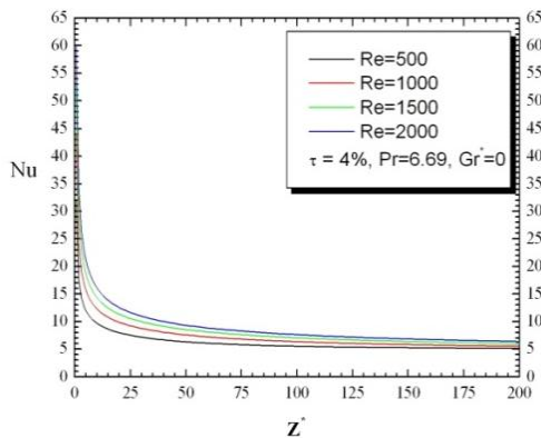
Fig. 5. The Nusselt number profiles along the annulus for the forced convection case.
