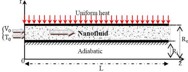
Fig. 1. The physical model and the correspondent geometry.
