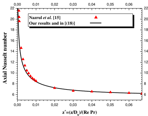
Fig. 2. Axial evolution of the circumferentially mean axial Nusselt number; A comparison with the results of [15].
