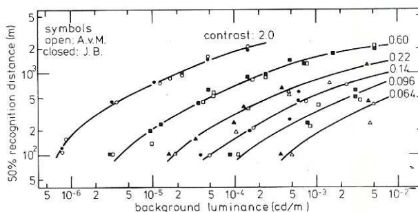
Fig. 5. Main results. Recognition distances as a function of background luminance as parameter. See text for definition of contrast.
