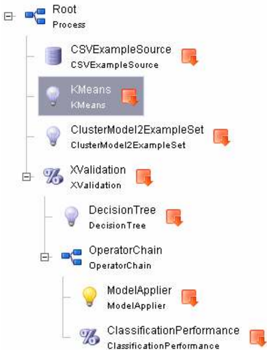
Fig. 1. Snapshot of the Operator Tree Used
