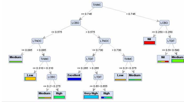
Fig. 7. Decision Tree Generated
