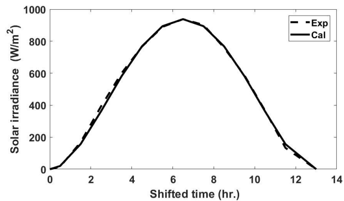
Figure 4. Comparison between experimental [13] and computed values (Equation (9)) for the incident solar irradiance ( \text{W}/\text{m}^2 ) for Makkah (Saudi Arabia).
