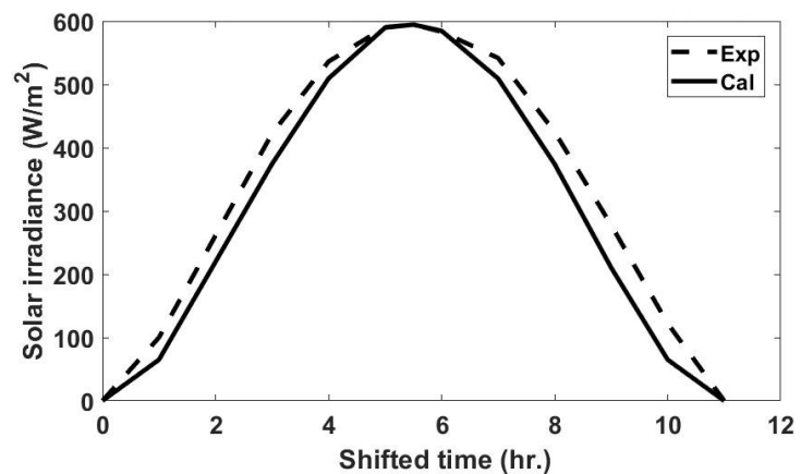
Figure 2. Comparison between experimental [7] and computed values (Equation (9)) for solar irradiance ( W/m^2 ) Hong Kong (China).
