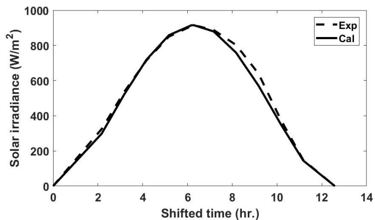
Figure 3. Comparison between experimental [12] and computed values (Equation (9)) for solar irradiance ( W/m^2 ) Jeddah (Saudi Arabia).
