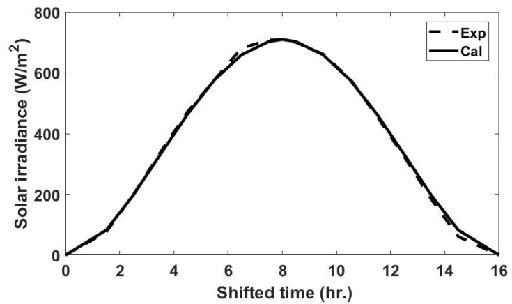
Figure 1. Comparison between experimental [9] and computed values (Equation (9)) for the incident solar irradiance ( W/m^2 ) for Barcelona (Spain).
