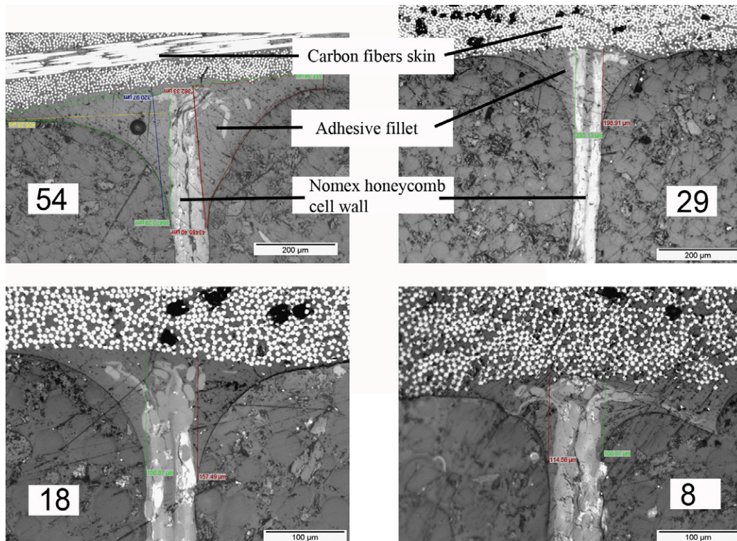
Fig. 12. Resin fillet with 54, 29, 18 and 8 g/m 2 adhesive. The size increases with adhesive weight. The end of the honeycomb cell walls is crushed, and this distorts the shape of the meniscus, especially at low adhesive weight. Note that the scale is different on the two lower micrographs.
