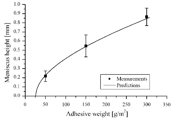
Fig. 16. Meniscus height predicted as a function of adhesive weight and contact angles. The contact angle with the carbon was considered as 0° and with the Nomex as 14°. The corresponding shape factor is \alpha = 0.52 . The adhesive weight M_0 which is not in the meniscus is considered as 26 g/m 2 .
