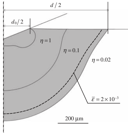
Fig. 6 Contours of equivalent plastic strain rate \dot{\bar{\epsilon}} at 1600 s. The CV is indicated by the area in gray. The dashed line shows the contour line for equivalent plastic strain \bar{\epsilon} = 2 \times 10^{-3} .
