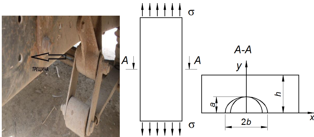
Fig. 4. Corrosion-fatigue crack of the vehicle's carrier [23] and the scheme of loading the plate with a surface semi-elliptic crack [15]
