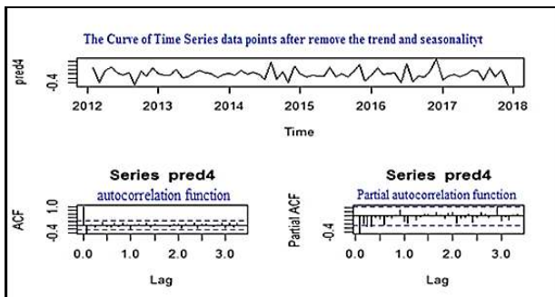
Fig.5. graphical procedures for a stable time Series after removing the trend and seasonality
