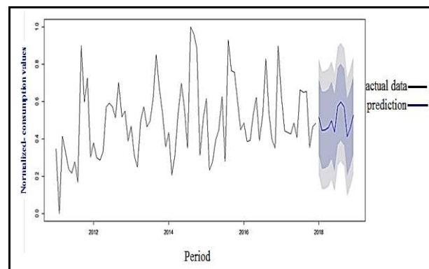
Fig.8. ARIMA best prediction result for 2018
