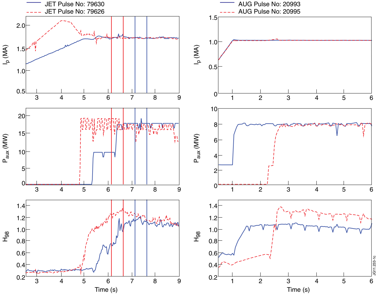
Figure 1: Temporal evolution of total plasma current (upper row), total auxiliary heating power P_{aux} = P_{NBI} + P_{ICRH} (center row), and H98 confinement factor (lower row) for the JET pair 79626/79630 (left panels) and AUG pair 20993/20995 (right panels).
