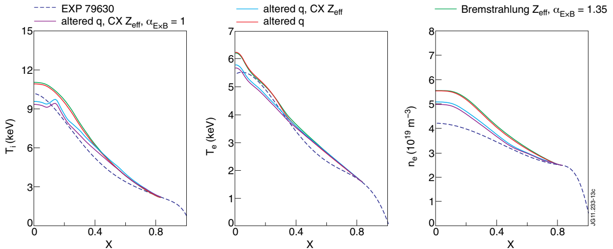
Figure 13: Results of combined heat and particle transport GLF23 simulations for JET 79630, testing the sensitivity of the results to Z_{\text{eff}} and the \alpha_{\text{ExB}} parameter. Progressive results for T_i (left panel), T_e (center panel), and n_e (right panel) are shown where the experimental profile is compared to: the original 79630 simulation with Bremsstrahlung Z_{\text{eff}} and \alpha_{\text{ExB}} = 1.35 , a simulation where the q -profile is substituted with the q -profile obtained with lowered Z_{\text{eff}} profiles, additionally reducing Z_{\text{eff}} itself in the predictive simulation to the CX measured Z_{\text{eff}} profile, and finally additionally switching the \alpha_{\text{ExB}} parameter to 1.
