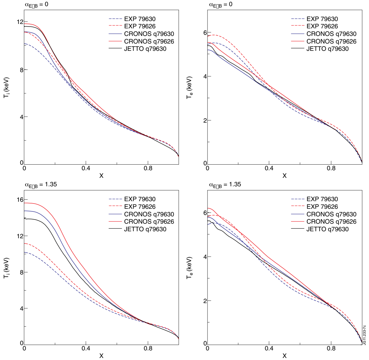
Figure 7: Results of heat transport only GLF23 simulations for JET Pulse No: 79630, comparing q -profile inputs from both Pulse No's: 79630 and 79626. T_i profiles are on the left column. T_e profiles are on the right column. Results with both no E \times B suppression (top row) and full E \times B suppression (bottom row) are shown. JETTO/GLF23 simulation results are also shown, to benchmark the CRONOS/GLF23 results.
