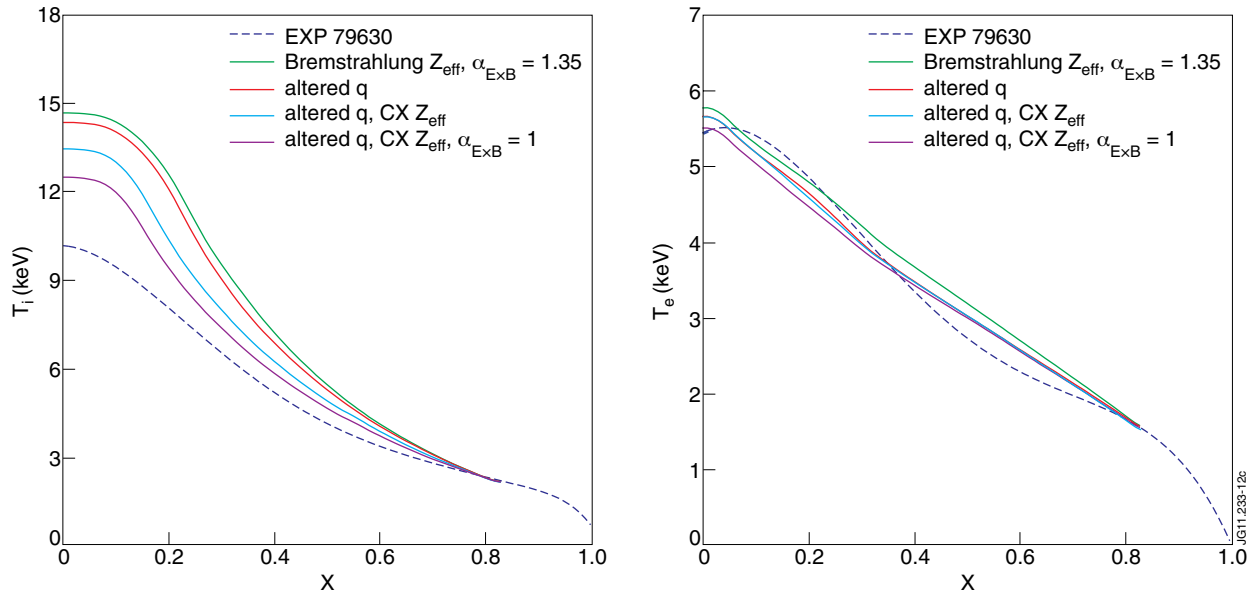
Figure 12: Results of heat transport GLF23 simulations for JET 79630, testing the sensitivity of the results to Z_{\text{eff}} and the \alpha_{\text{ExB}} parameter. Progressive results for T_i (left panel) and T_e (right panel) are shown where the experimental profile is compared to: the original 79630 simulation with Bremsstrahlung Z_{\text{eff}} and \alpha_{\text{ExB}} = 1.35 , a simulation where the q -profile is substituted with the q -profile obtained with lowered Z_{\text{eff}} profiles, additionally reducing Z_{\text{eff}} itself in the predictive simulation to the CX measured Z_{\text{eff}} profile, and finally additionally switching the \alpha_{\text{ExB}} parameter to 1.
