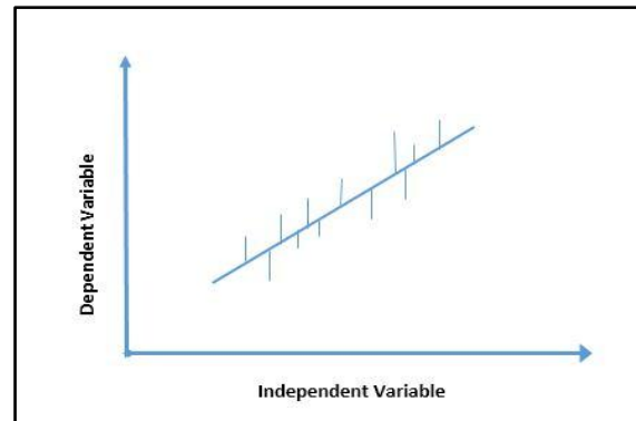
Figure 4: Regression Model
