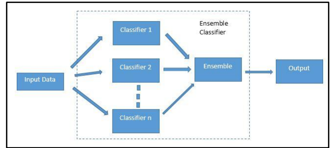
Figure 7: Ensemble Classifier
