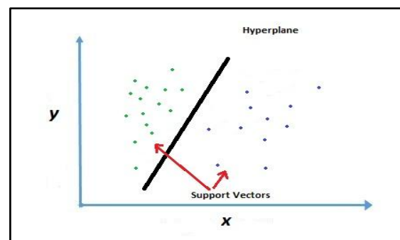
Figure 9: Support Vector Machine
