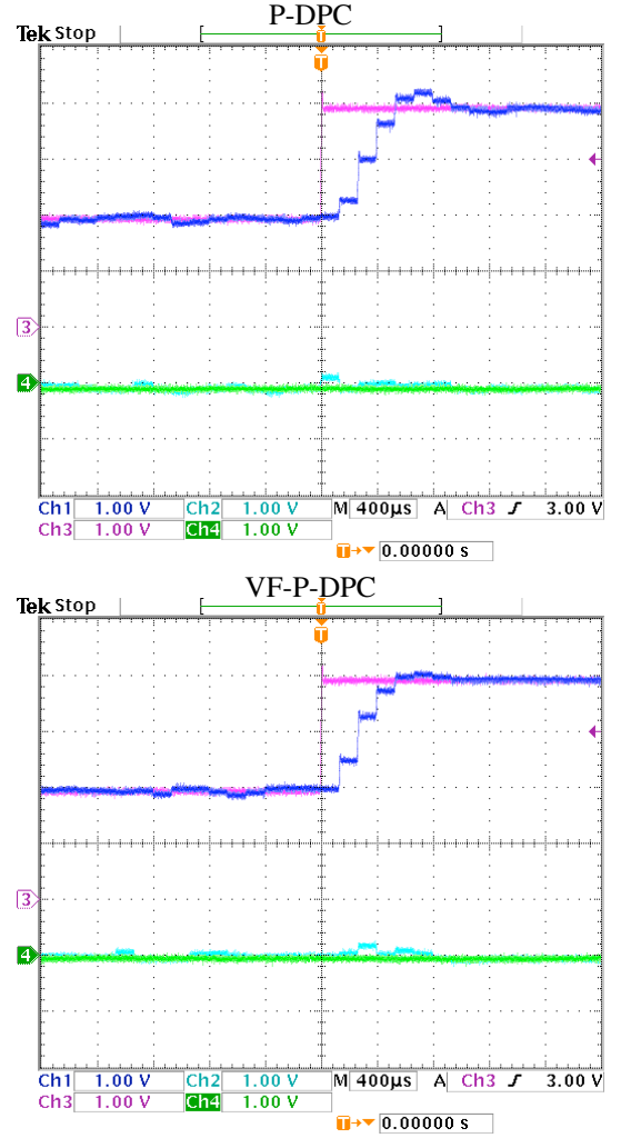
Fig. 15. Experimental tracking performance of active power control for command change from 1 kW to 2 kW. Upper figure: constant switching frequency Predictive Direct power Control (P-DPC) with grid voltage sensors, Lower figure: constant switching frequency Virtual Flux based Predictive Direct power Control (VF-P-DPC) without grid voltage sensors. From the top: commanded and measured active and reactive powers.
