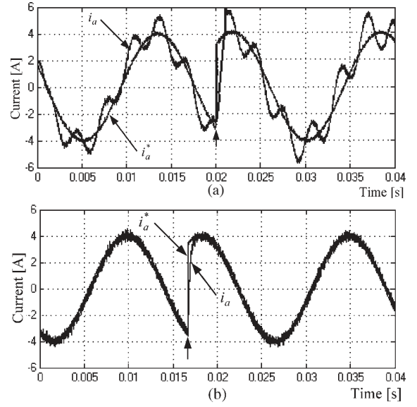
Fig. 9. Experimental results for the deadbeat current control. (a) Conventional deadbeat current controller implemented in a full digital system (without any compensation). (b) Modified deadbeat current controller proposed in [34].
