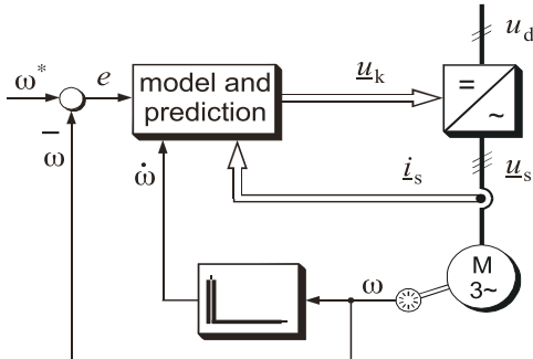
Fig. 5. Direct Speed Control (DSPC).
