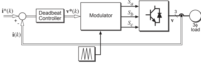
Fig. 7. Deadbeat current control.
