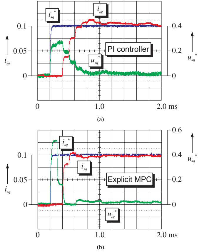
Fig. 12. Experimental tracking performance of current control: (a) with PI controllers designed according to Symetrical Optimum, (b) with Model Predictive Controller (MPC) [44].
