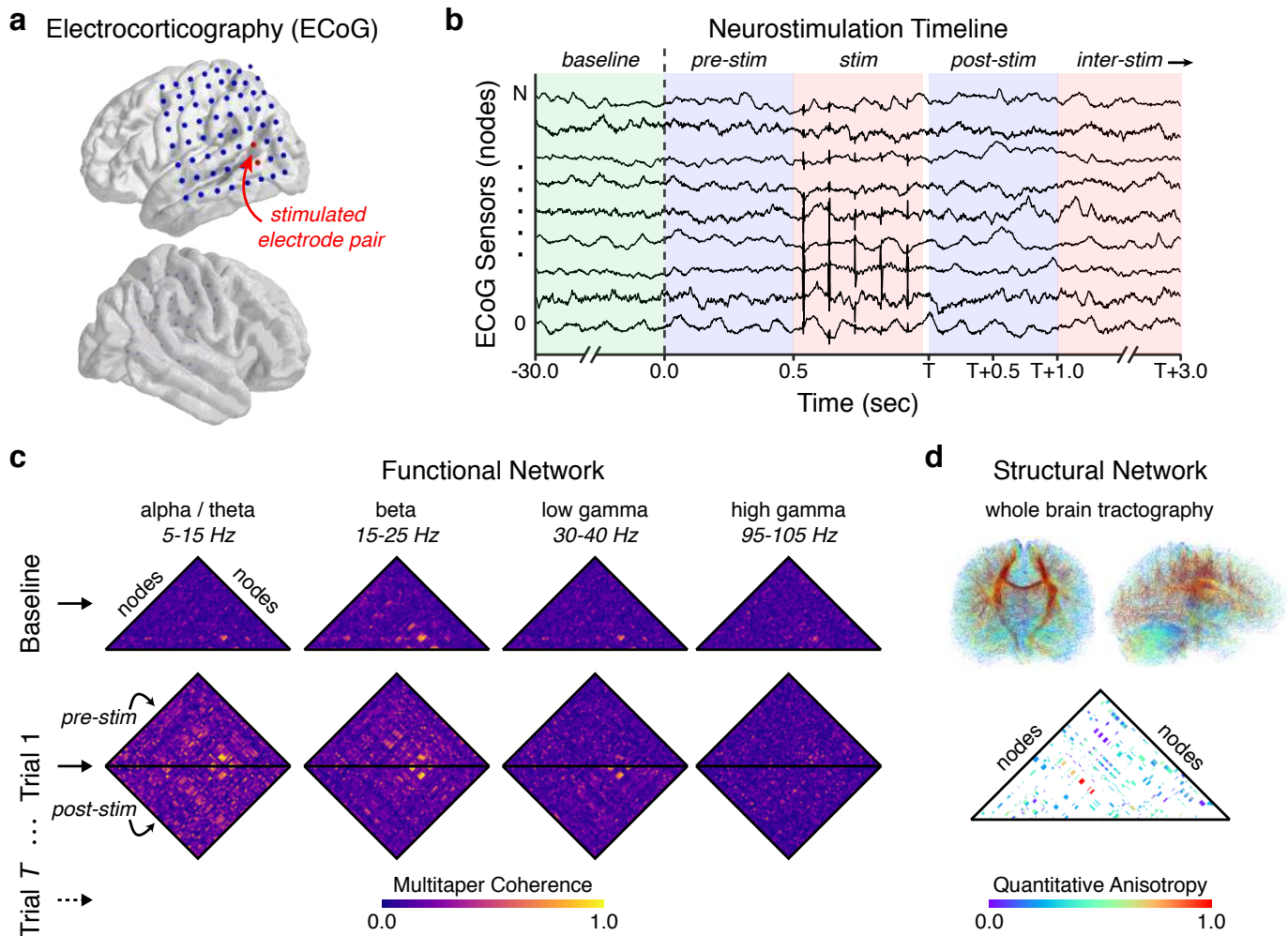
Figure 1: Measuring network response to targeted, intracranial neurostimulation. (a) We record the electrocochogram (ECoG) in 94 patients with drug-resistant epilepsy across 8 clinical institutions using intracranial sensors implanted in cortical and subcortical brain structures. To evoke a network response, we stimulate adjacent electrode pairs using a charge-balanced, biphasic current source with a square waveform of variable amplitude, frequency, and duration. (b) For each experimental session, we select a stimulation location and collect the following epochs of ECoG activity: (i) thirty seconds of baseline activity before any stimulation is given, (ii) one half-second of activity before a stimulation trial, and (iii) two consecutive and non-overlapping half-second windows of activity after a stimulation trial. A stimulation trial is defined by a combination of pulse frequency, amplitude, and duration, and consecutive stimulation trials are separated by an inter-stimulation interval drawn from a uniform random distribution ranging from 2.75 seconds to 3.25 seconds. (c) We measure the impact of neurostimulation on functional network architecture by constructing dynamic graph models in which intracranial sensors are represented by nodes and the functional interactions between intracranial sensors are represented by edges . To infer functional interactions, we calculate the multitaper coherence between each pair of ECoG signals in non-overlapping, half-second time windows for each baseline epoch, pre-stimulation epoch, and post-stimulation epoch in the following four frequency bands: (i) alpha/theta (5-15 Hz), (ii) beta (15-25 Hz), (iii) low gamma (30-40 Hz), and (iv) high gamma (95-105 Hz) [63, 57]. (d) To examine how structural connectivity constrains functional network reconfiguration to neurostimulation, we also construct a static graph model of the brain's structural network by applying deterministic tractography to each subject's diffusion tensor imaging data.
