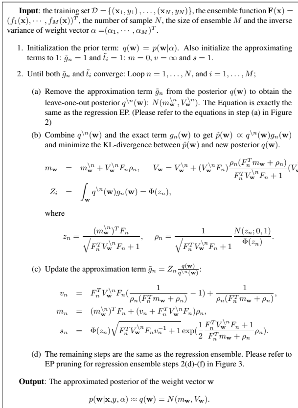
Fig. 4. Expectation Propagation for Classification Ensembles
