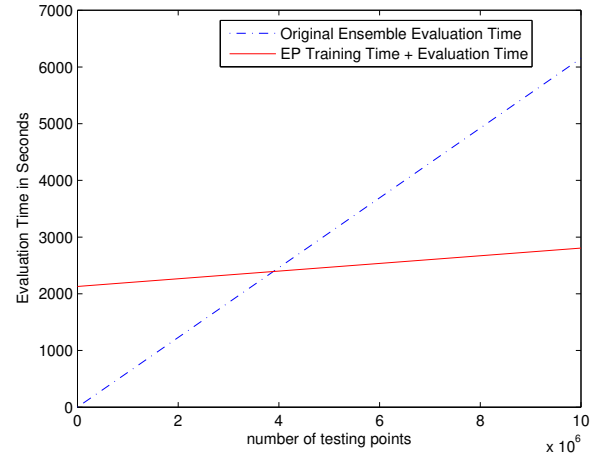
Fig. 10. Comparison of evaluation time of each pruning method averaged.
