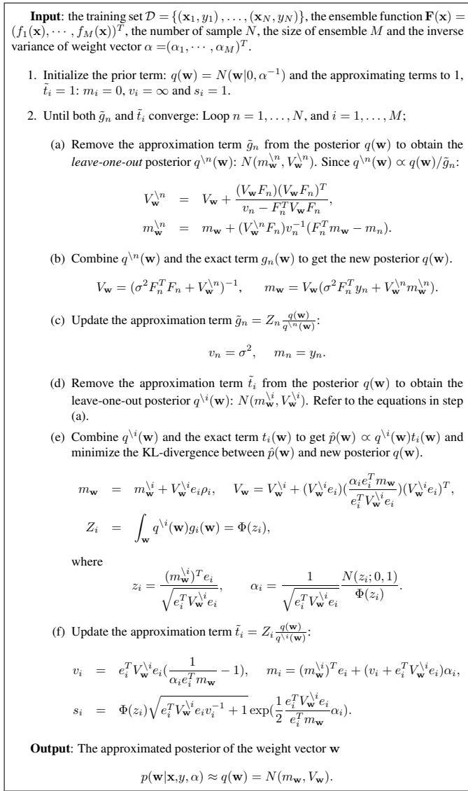
Fig. 3. Expectation Propagation for Regression Ensembles
