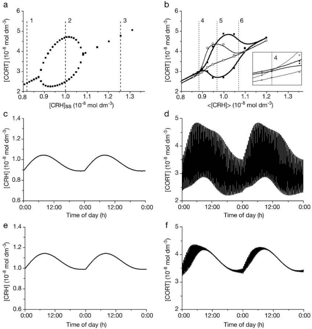
Fig. 5 (a) Bifurcation diagram showing the ultradian cortisol dynamics as a function of [CRH] SS . Single points denote stable stationary states, whereas the oscillatory states are presented by pairs (minima and maxima) of cortisol concentrations in the ultradian oscillations. Vertical lines indicate three different dynamic states: (1) at low CRH levels, [CRH] SS = 0.82 \cdot 10^{-8} mol \text{dm}^{-3} , a low cortisol concentration steady state, denoted as 1 in Fig. 1b, is established. (2) At [CRH] SS = 1.00 \cdot 10^{-8} mol \text{dm}^{-3} , ultradian cortisol oscillations, denoted as 2 in Fig. 1b, are established. (3) At high CRH levels, [CRH] SS = 1.26 \cdot 10^{-8} mol \text{dm}^{-3} , a high cortisol concentration steady state, denoted as 3 in Fig. 1b, is established. (b) Bifurcation diagrams showing the ultradian cortisol dynamics as a function of <[CRH]>. In a model with circadian regulation, nocturnal (■) and daytime (○) ultradian cortisol oscillations are different. Vertical lines indicate three different dynamic states: (4) at low <[CRH]> = 0.88524 \cdot 10^{-8} mol \text{dm}^{-3} (basic physiological conditions), ultradian oscillations are observed during the daytime whereas the amplitude of nocturnal ultradian oscillations is very small (this region is magnified in the insert; corresponding CORT time series are shown in Fig. 1d). (5) At <[CRH]> = 0.97 \cdot 10^{-8} mol \text{dm}^{-3} , ultradian oscillations with relatively large amplitudes are observed during daytime and at night (corresponding CRH and CORT time series are shown in Fig. 5c and 5d, respectively). (6) At <[CRH]> = 1.07 \cdot 10^{-8} mol \text{dm}^{-3} , the ultradian oscillatory dynamics is reversed, showing large-amplitude cortisol oscillations at night, while small-amplitude cortisol oscillations during daytime (corresponding CRH and CORT time series are shown in Fig. 5e and 5f). In all cases, d_2 = 0.957 .
