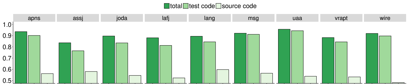
Fig. 15 Comparison of source code features and test code features. The y axis represents the AUC values. Different bars indicate the total effectiveness, as well as the effectiveness with only source code features or test code features. Test code related features perform much better than source code related features.
