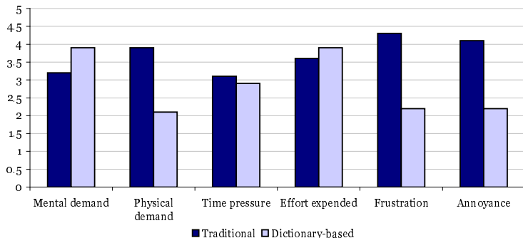
Figure 6: NASA TLX Results
