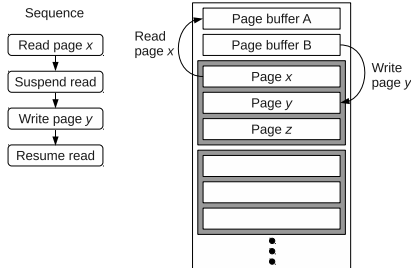
Fig. 8: An example of preempting an on-going flash operation with the suspend command.
