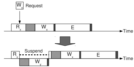
Fig. 9: Operation sequence of fully preemptible GC.
