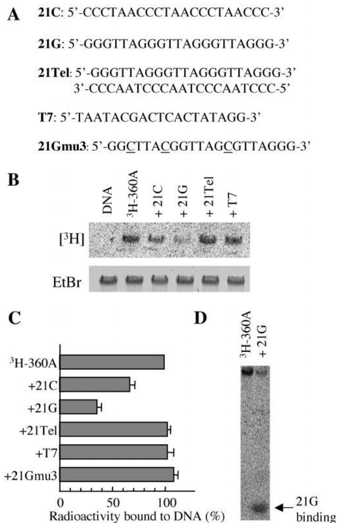
Figure 2. Specific binding of ^3\text{H} 360A to telomeric G-overhang. (A) Sequence of the oligonucleotide competitor used. (B) Binding of ^3\text{H} -360A (1 nM) to purified A549 genomic DNA after agarose gel electrophoresis in the absence or presence of 1 \mu\text{M} oligonucleotide competitors (+21C, +21G, +21Tel, +T7) or DNA, control DNA without ^3\text{H} -360A. [ ^3\text{H} ], radioactive signal of the gel; Et-Br, ethidium bromide staining of the gel. (C) Quantification of the ^3\text{H} -360A binding to the genomic DNA. The radioactivity signal is normalized relative to the Et-Br signal, defined as 100% for 1 nM ^3\text{H} -360A without competitors. The results corresponded to at least three independent experiments (mean \pm SD). (D) In the presence of 21G (1 \mu\text{M} ), most of the ^3\text{H} 360A radioactivity was detected at the position of the oligonucleotide (indicated by an arrow at the bottom of the gel).
