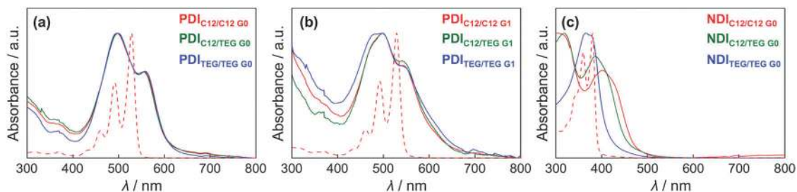
Fig. 5 Absorption spectra of the (a) \text{PDI}_{\text{G0}} , (b) \text{PDI}_{\text{G1}} , and (c) \text{NDI}_{\text{G0}} derivatives in the film state (solid line) together with the spectra of (a) \text{PDI}_{\text{C12/C12 G0}} , (b) \text{PDI}_{\text{C12/C12 G1}} , and (c) \text{NDI}_{\text{C12/C12 G0}} in \text{CHCl}_3 (dashed line) at 25 °C.
