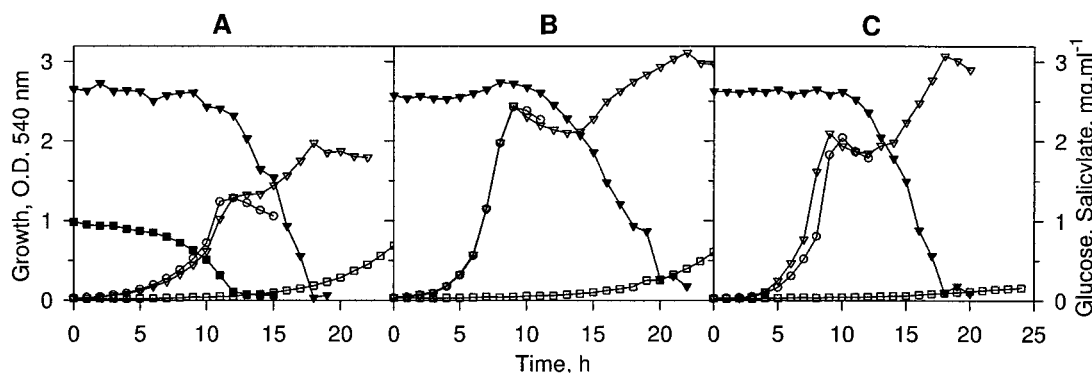
FIG. 2. Growth profile of P. putida CSV86 on 0.1% aromatics plus 0.25% glucose ( \nabla ), 0.1% aromatic compounds ( \circ ), or 0.25% glucose ( \square ). Aromatics used were salicylate (A), benzyl alcohol (B), and benzoate (C). Cells grown on the respective aromatic compound were used as an inoculum. Measured salicylate ( \blacksquare ) and glucose ( \blacktriangledown ) concentrations in the culture media are shown.
