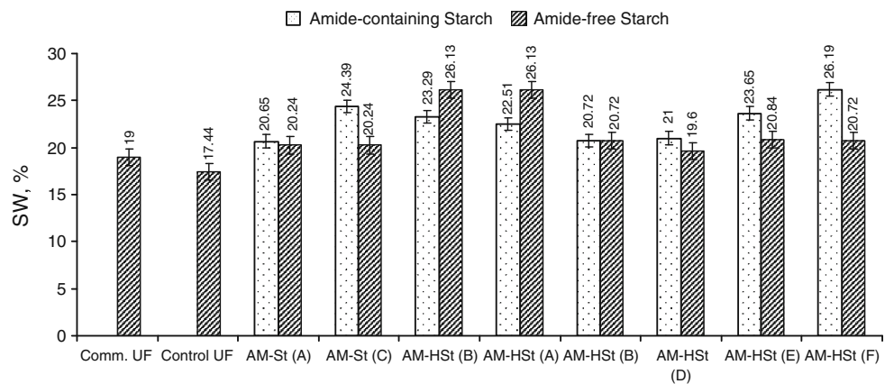
Fig. 9 Effect of modified UF by starch- based biopolymers on water swelling performance of sugar cane fiber bagasse composites
