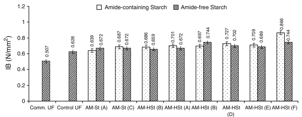
Fig. 8 Effect of modified UF by starch- based biopolymers on internal bond (IB) strength of sugar cane fiber bagasse composites
