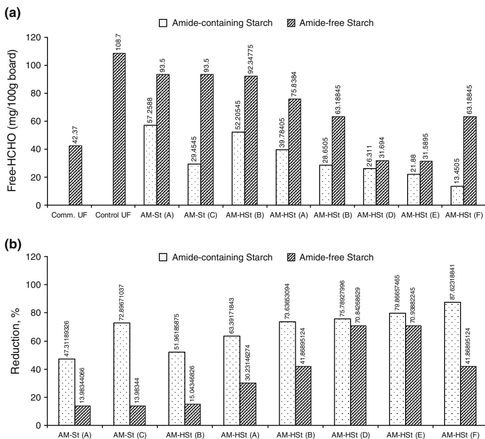
Fig. 6 Effect of modified UF by starch- based biopolymers on free-HCHO emitted from bagasse composites
