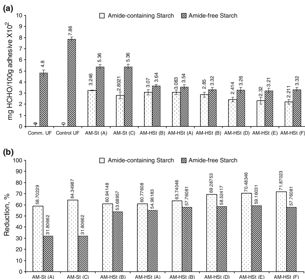
Fig. 1 Effect of modified UF by starch- based biopolymers on free-HCHO of produced adhesives. a Free-HCHO of unmodified and modified UF adhesives, and b Reduction of free-HCHO of modified UF/unmodified one
