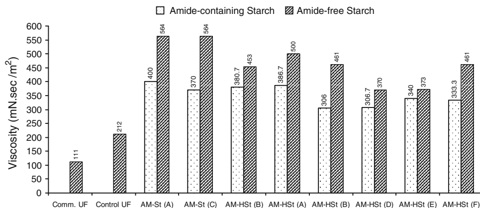
Fig. 3 Effect of modified UF by starch- based biopolymers on viscosity of modified UF—adhesive
