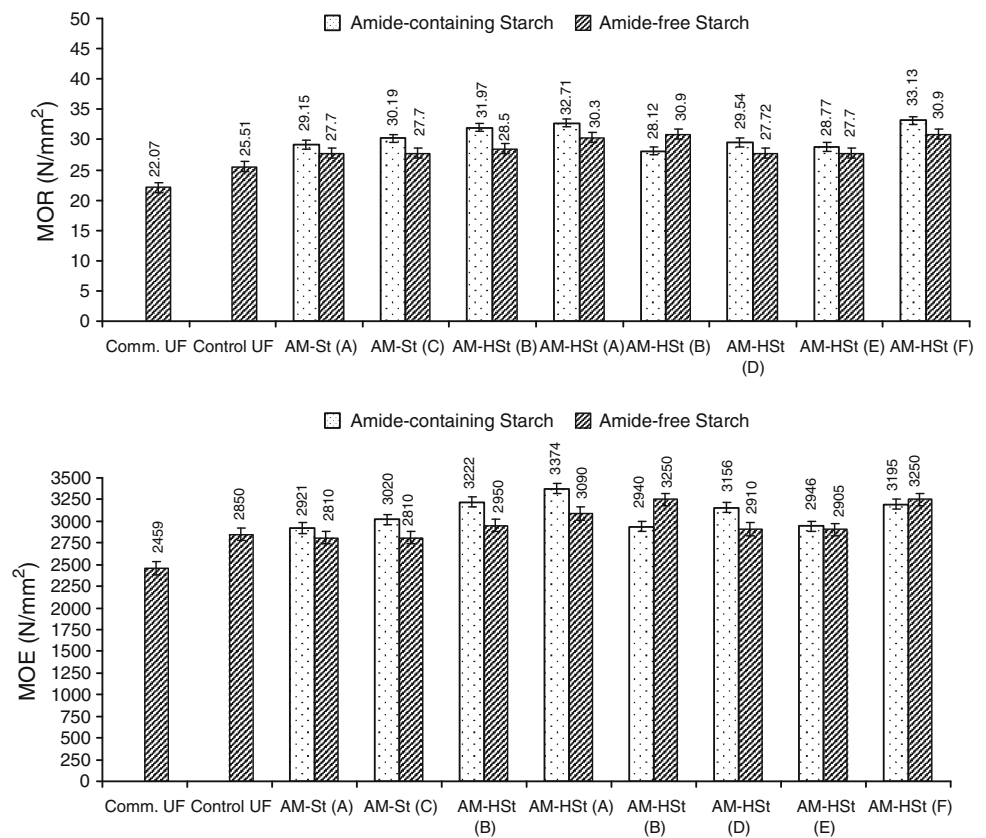
Fig. 7 Effect of modified UF by starch- based biopolymers on static bending properties (MOR & MOE) of sugar cane fiber bagasse composites produced
