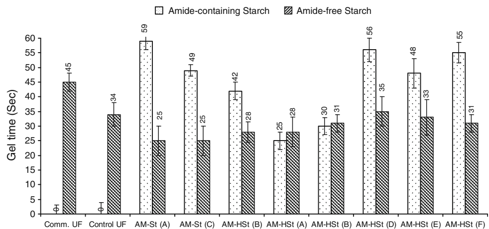
Fig. 5 Effect of modified UF by starch- based biopolymers on gel time of modified UF—adhesives
