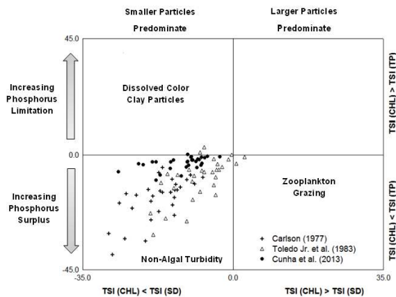
Figure 3. Graphic showing differences [TSI (Chl a ) - TSI (TP)] versus [TSI (Chl a ) - TSI (SD)] and possible interpretation on deviations of rates of the Trophic State Index (TSI) of Carlson (1977), Toledo Junior et al. (1983) and Cunha et al. (2013) from data obtained in the Pereira de Miranda Reservoir (Pentecoste, Ceará, Brazil), 2012 and 2013. Source: Adapted from Carlson and Havens (2005).
