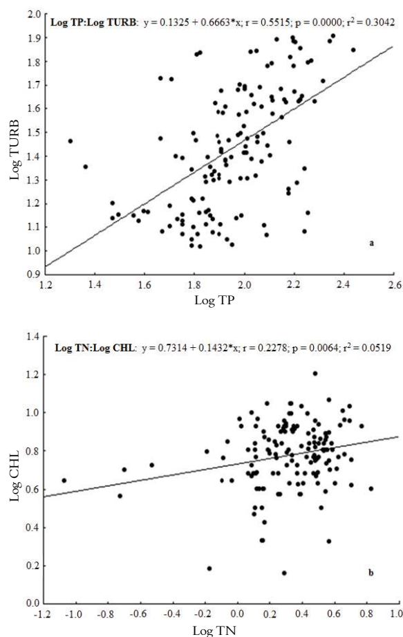
Figure 4. Linear regression analysis for significant correlations ( p < 0.05 ) between log-transformed data from turbidity and total phosphorus (a) and chlorophyll a , and total nitrogen (b) from data obtained in the Pereira de Miranda Reservoir (Pentecoste, Ceará, Brazil), 2012 and 2013. Source: Researcher, 2014.
