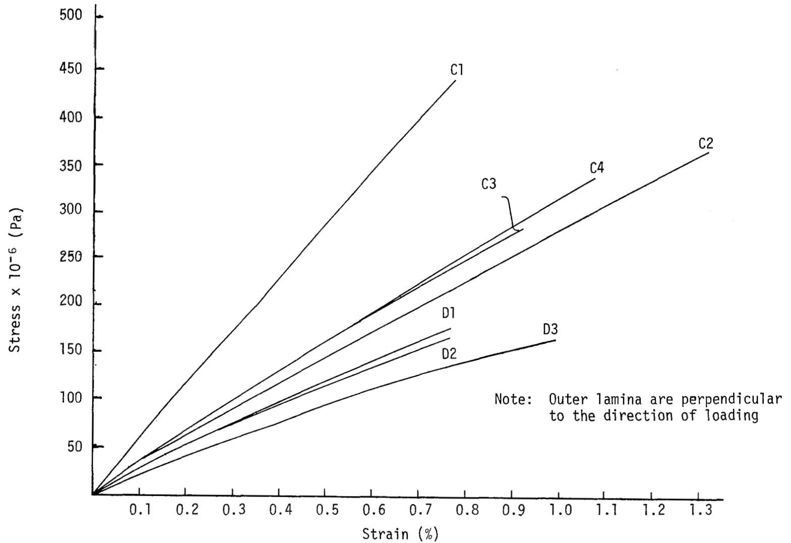
Figure 12. Tensile Stress/Strain Curves ( E_{11} ) of Eight Ply Multidirectional Laminates of Groups C and D
