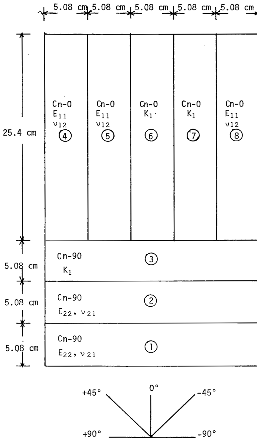
Figure 2. Coupon Designation for Panels in Groups C and D
